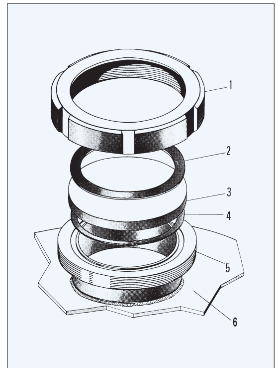
Exploded view of an MV series Weld Neck sightglass fitting
